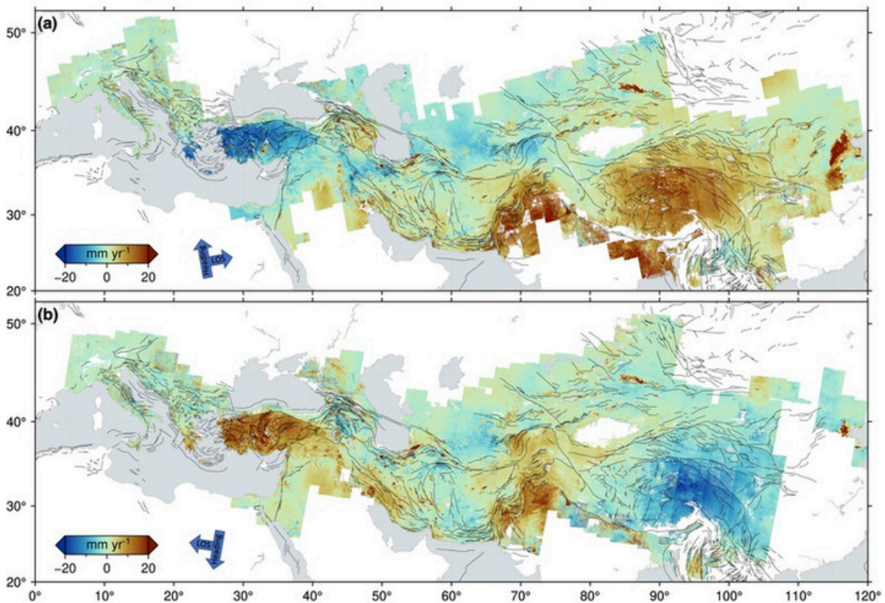
Figure 1: Average mosaic of referenced line of sight velocities for the Alpine Himalayan Belt on (a) ascending and (b) descending orbital heading directions, with positive values indicating motion away from the satellite. Active fault traces (black lines) are from Styron & Pagani (2020).
